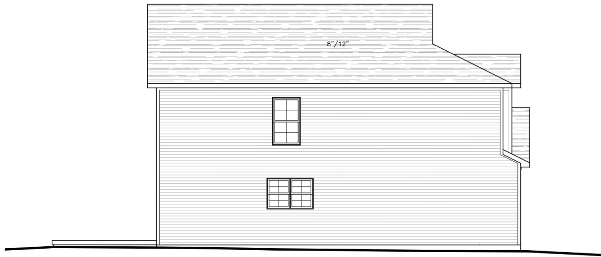
LEFT ELEVATION 1/8" = 1'-0"
