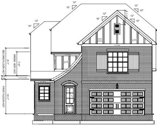
1 Front Elevation 1/8" = 1'-0"
