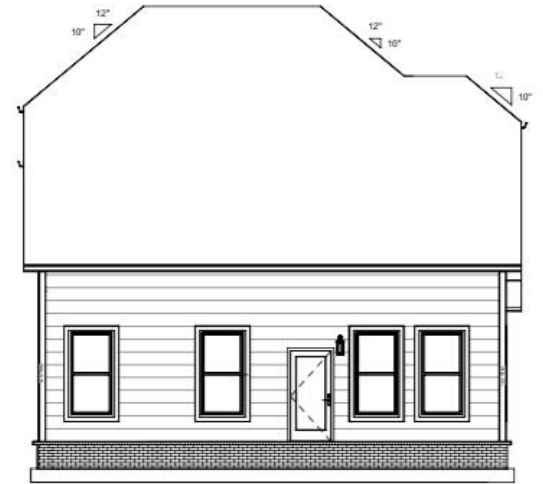
2 Rear Elevation 1/8" = 1'-0"
